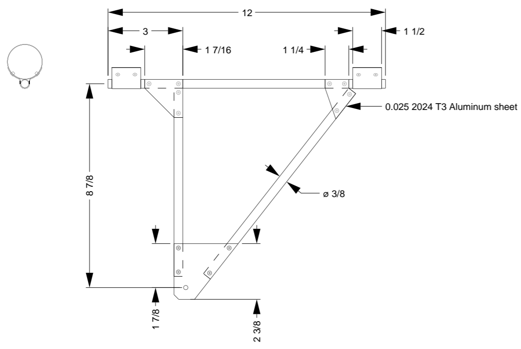
CANARD SUPPORT FRAME
