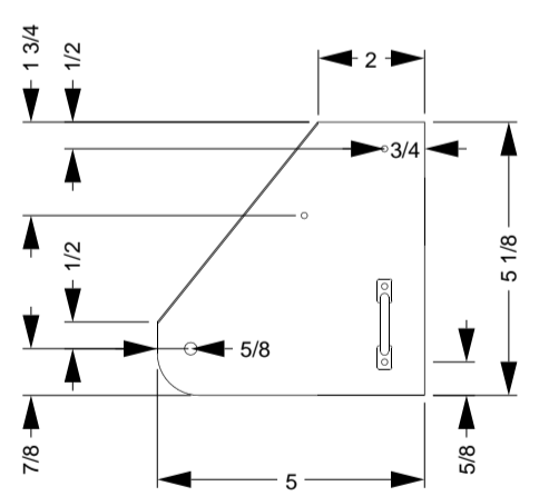
FORWARD WHEEL BRACKET 0.026 Aluminum sheet
