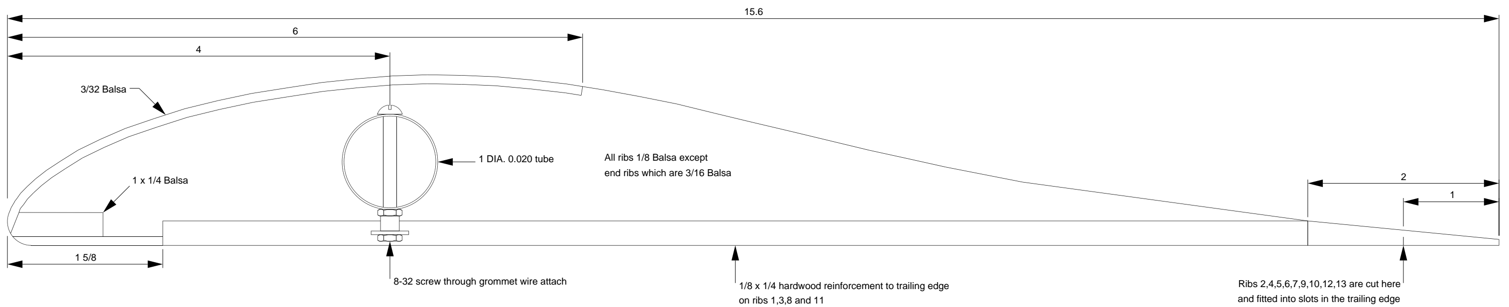
SECTION A-A (Typical reinforced rib)
