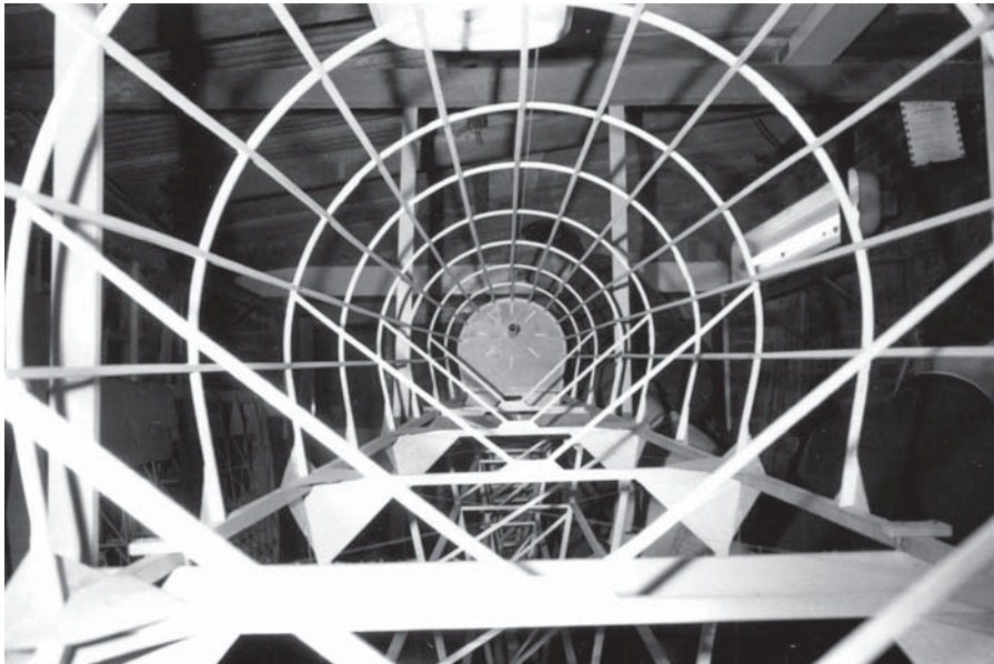
Top fairing, laminated balsa hoops, I-section stringers
