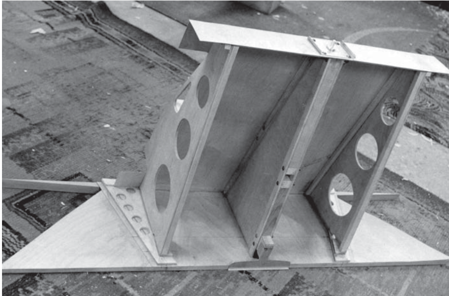
Wing centre box sub assembly, ply ribs for main attachments
