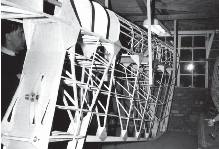
Rear fuselage, triangular balsa frames, spruce longerons
