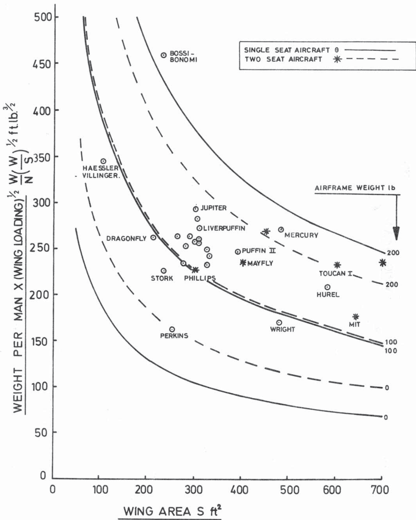
Fig 7: Man-Powered Aircraft Relative Performance Structural Factor
