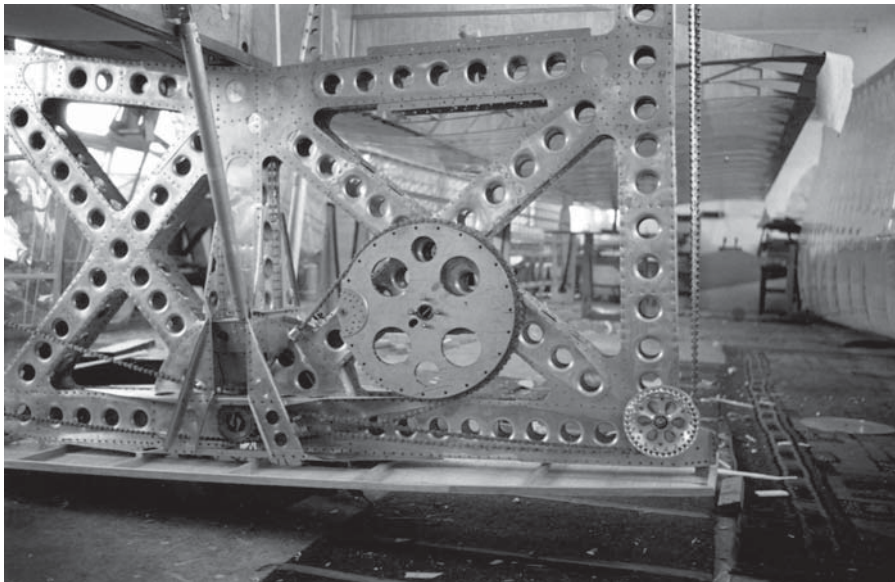
Wing attachment, sprocket wheel, idler, and al aly chains
