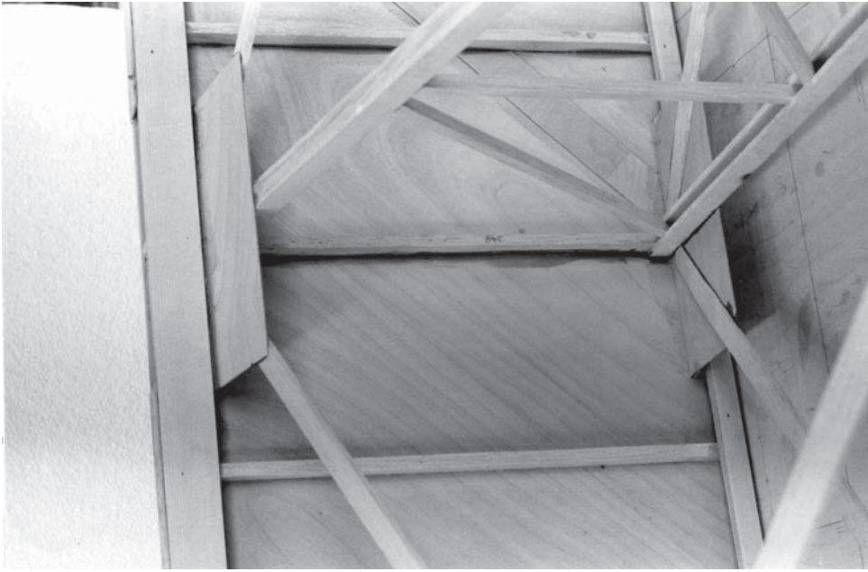
Twin flange main spar with diagonal web and capping, balsa stiffeners, main ribs and spruce diagonal bracing.
