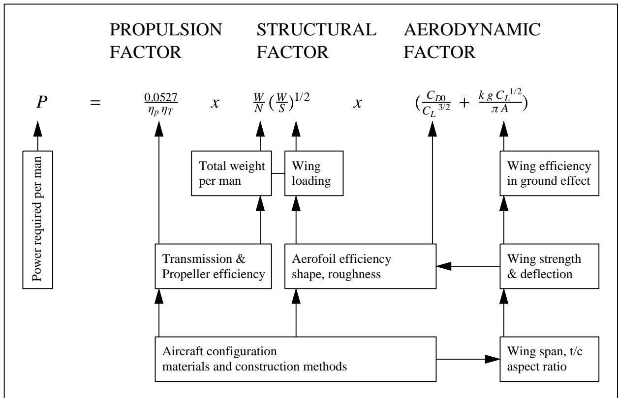
Fig 6: Structural Design Influence on Power Requirement
