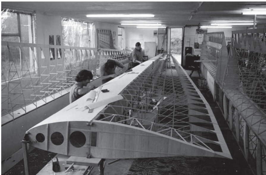
Polystyrene nose formers with sheeting and pre cut LE
