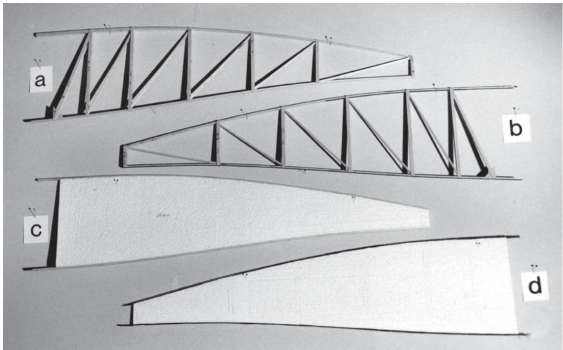
Experimental ribs suitable for a single seat aircraft. Total chord 1.5 m
