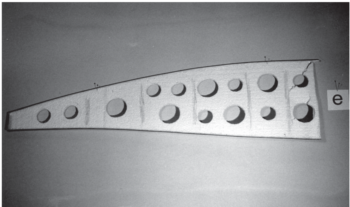
Rib (e) after modification by the introduction of lightning holes
