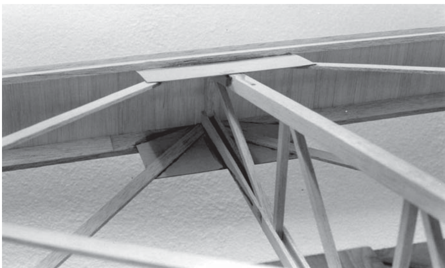
Balsa nose spar, ply gussets attach main ribs and bracing
