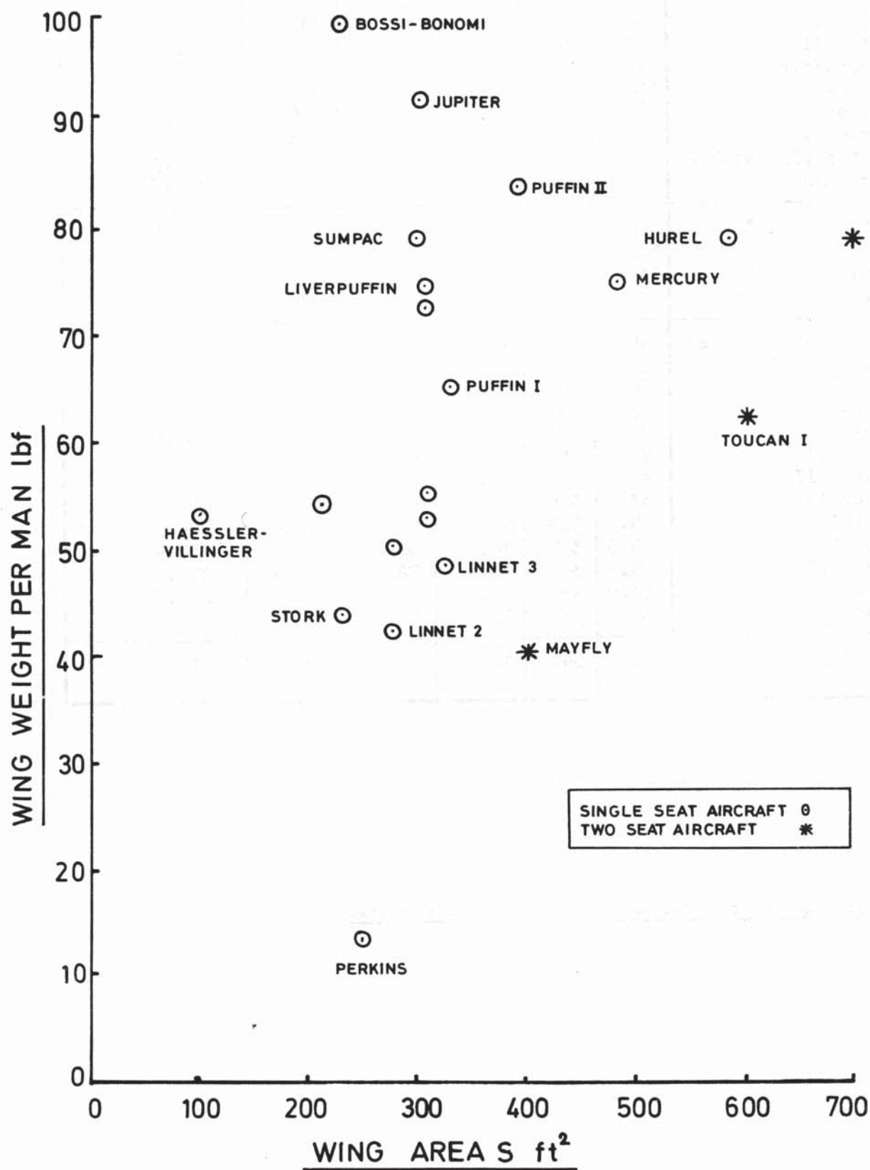
Fig 4: Man-Powered Aircraft Wing Weights
