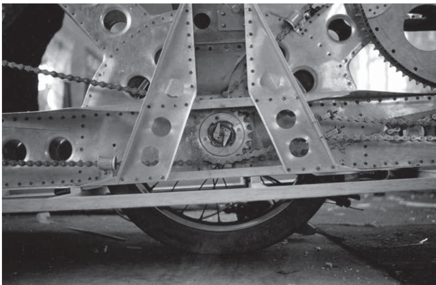
Chain drive to and from road wheel, free wheel clutch
